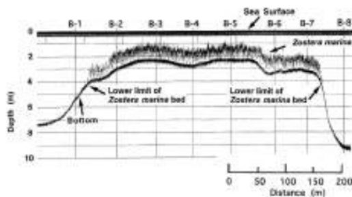
Fig. 11. Raw records of echo trace along a transect in Ajino Bay, Japan cited from Komatsu and Tatsukawa (1998). A depth of 0 m is the sea surface, which is not standardized to the depth relative to the mean sea level.
