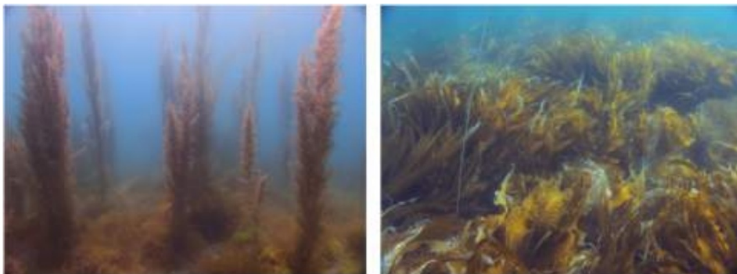
Fig. 2. Photos showing forests of brown algae, Stephanocystis hakodatensis (Yendo) Draisma, Ballesteros, Rousseau et Thibaut (left photo), and Saccharina japonica (Areschoug) Lane, Mayes, Druehl et Saunders var. religiosa (Miyabe) Yotsukura, Kawashima, Kawai, Abe et Druehl (right photo) off Kamoenai, west coast of Hokkaido, Japan.
