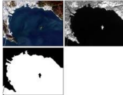
Fig. 16. LANDSAT 8 OLI images of true color (upper left), band 5 (upper right) and mask (lower) on Ajino Bay, Japan. The mask was produced from pixels with DN values of near-infrared band less than 7000.
