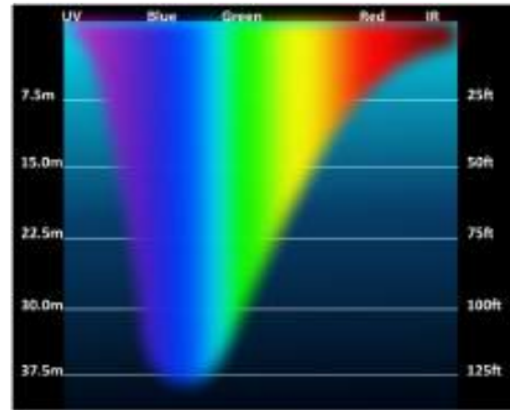
Fig. 3. Patterns of vertical penetration of light between ultraviolet and infrared into the water (courtesy of Prof. Tom Morris of Fullerton College).
